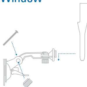
1. Assemble Mount
